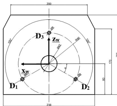
Fig. 10. Schematic view of the internal plate. Dimensions needed to calculate the coordinates of centres of the ball joints D_j, j = 1-3 are shown
