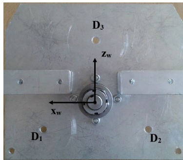
Fig. 2. An overview of the internal plate of the prototypical instrument for measurement of the linear and angular displacements of the steered wheel. Positions of the ball joints D_j , j = 1-3 and the Cartesian coordinate system connected with the plate is shown (The y_w - axis coincides with y - axis of the coordinate system connected with the external plate)
