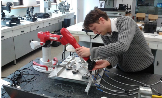
Fig. 8. The measurement of the coordinates of the ball joints H_i , i = 1(9) centres using the ROMER measuring arm
