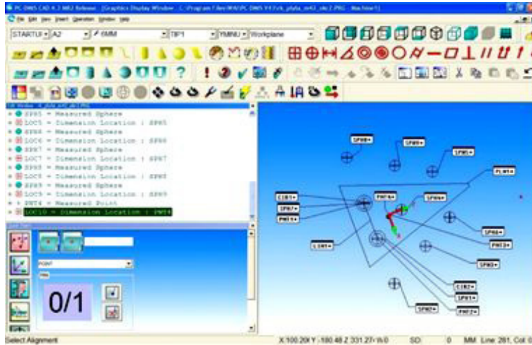
Fig. 9. Window of the computer program which recorded the measurements data. The coordinate system, objects that were used to build it (See Fig. 5) and the positions of ball joints, which coordinates were searched are shown (Symbols SPH1–SPH9)
