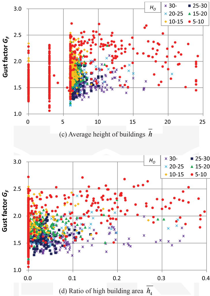
Fig. 7 (cont). Relationship between G_F and surface roughness classified into several height classes
