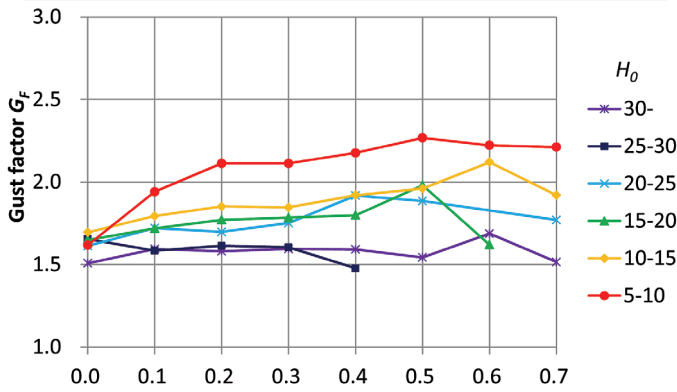
(b) Building volume ratio V_b
