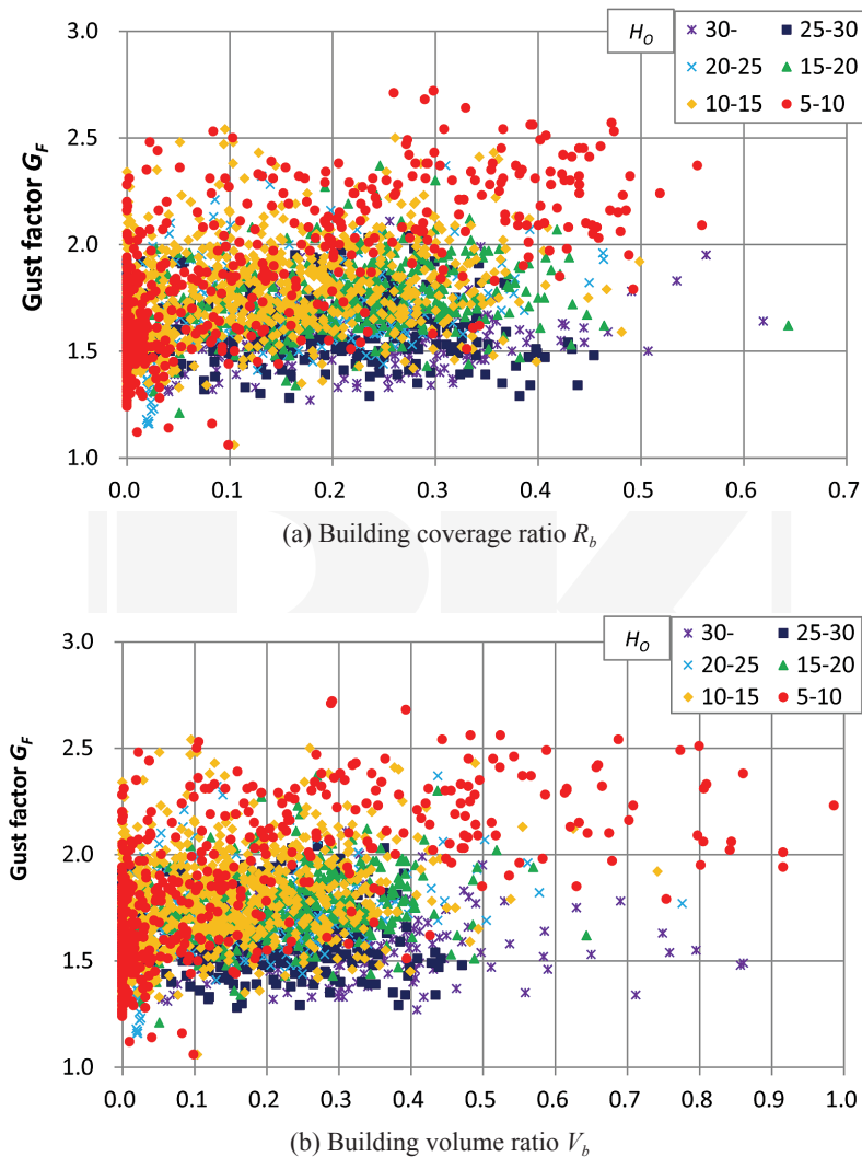
Fig. 7. Relationship between G_F and surface roughness classified into several height classes
