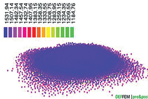
Fig. 6. Example temperature distribution of the computational domain (time 0.18009102709323876 s.)
