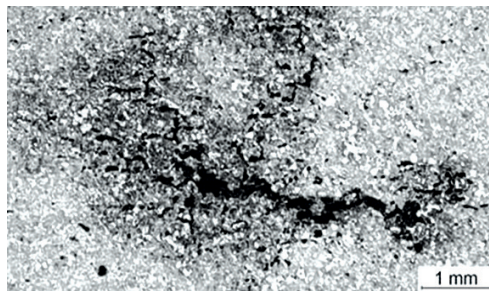
Fig. 4. Macrostructure of the sample centre with visible defects area after re-melting process at 1430°C
