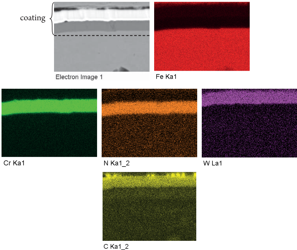
Fig. 1. Element distribution maps showing the chemical composition of the coating
