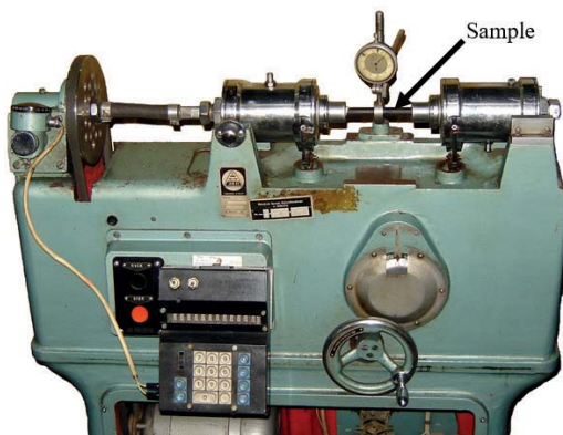
Fig. 5. The structure of a fatigue testing machine
