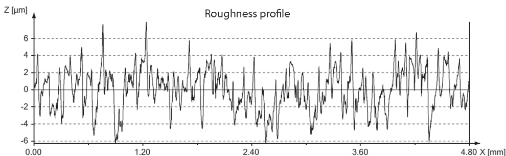
Fig. 2. Roughness profile of the shaft surface
