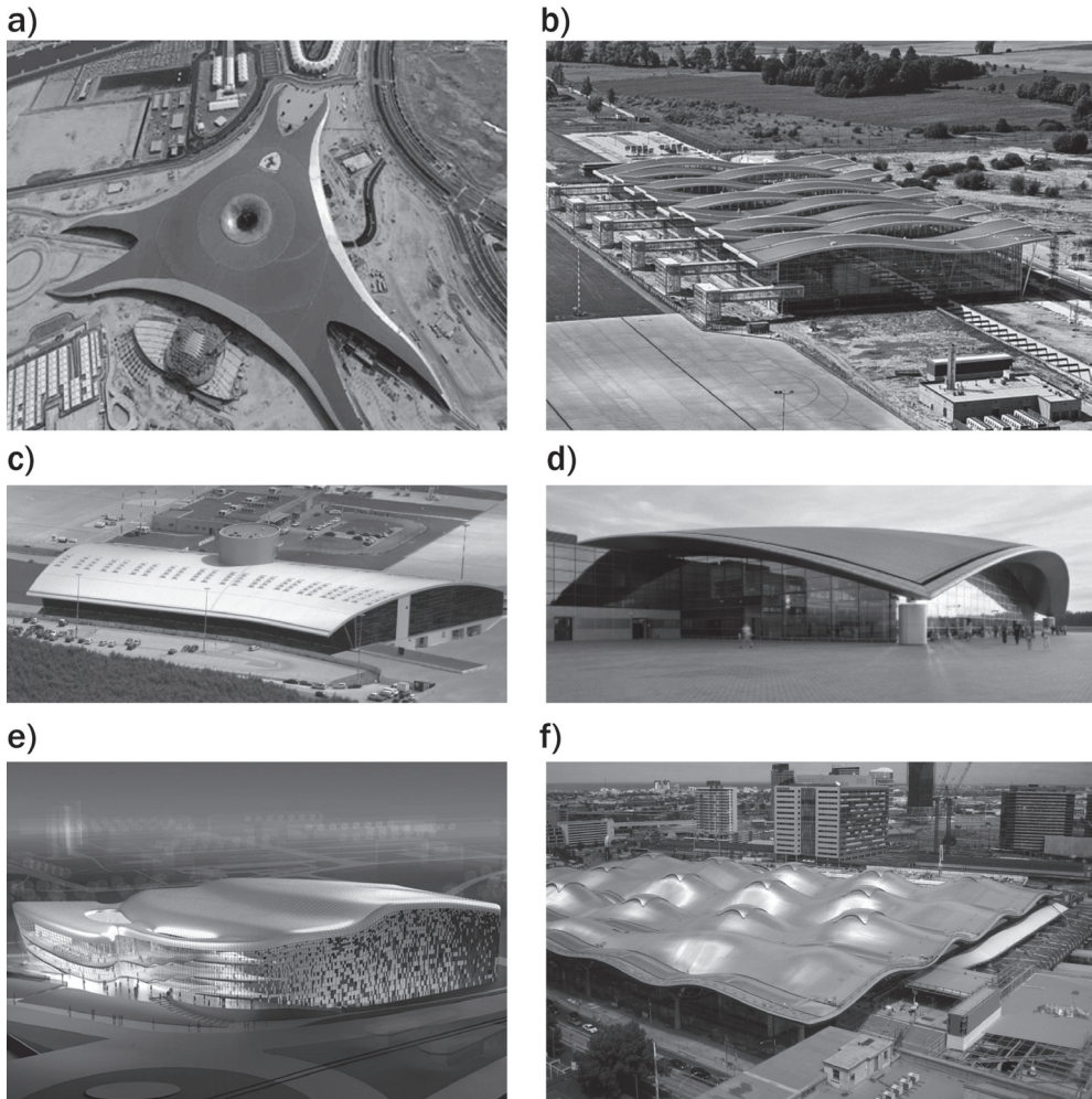
Ill. 1. Examples of roofs covered with self-supporting metal panels: a) Ferrari World Abu Dhabi [14], b) airport terminal in Wroclaw [18] c) airport terminal in Lodz [16], d) airport terminal in Rzeszow Jasionka [9], e) Convention Center in Krakow now under construction [11], f) Southern Cross Station Melbourne, Australia [17]
