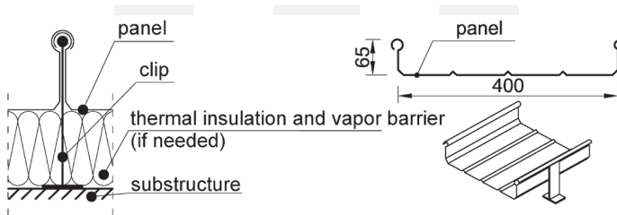
Ill. 2. Cover of the roof with self-supporting metal panels: components and sample shape of panel
