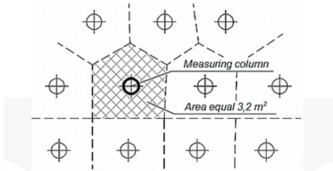
Fig. 13. Reference area for calculation of stress in the ground surrounding considered column
