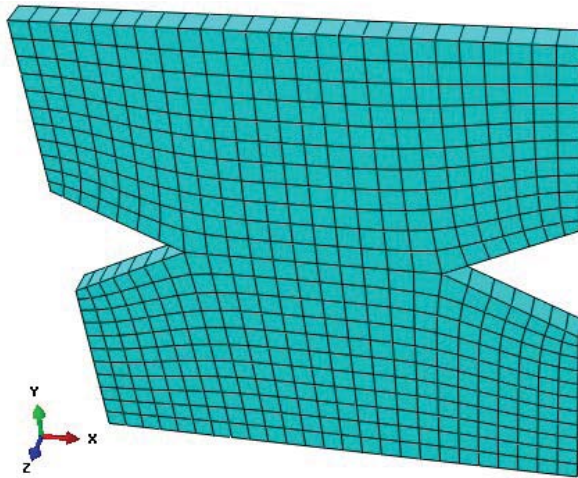
Fig. 3. Numerical model after discretisation (source: own study)
