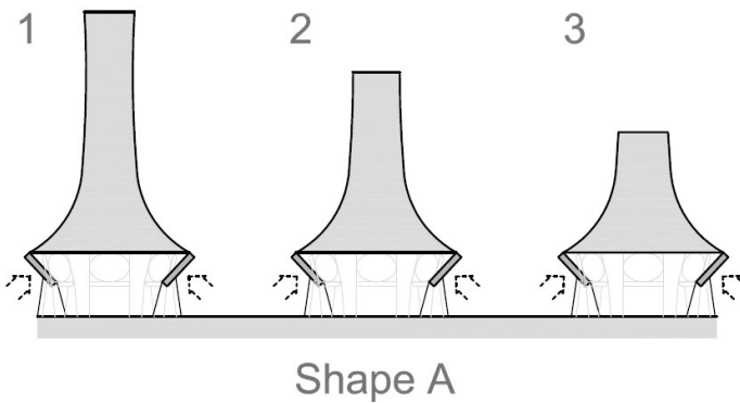
Fig. 4. Different variants of chimney shape A
