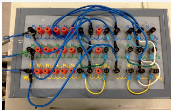
Fig. 1. Stator windings configuration panel
