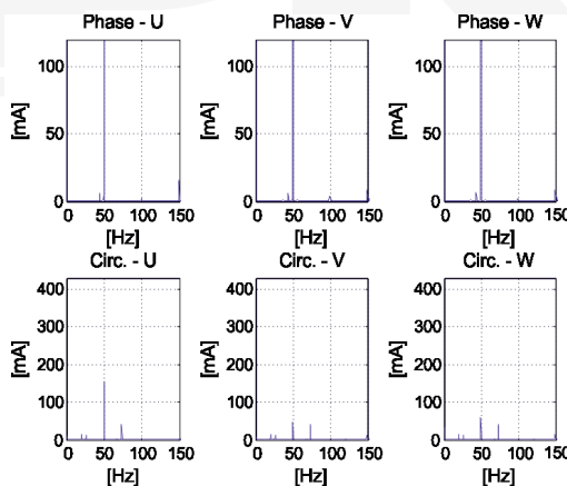
Fig. 4. Harmonics of phase currents [mA] (row above) and circulating currents [mA] (row below) – 30% of turns in the coil of the stator winding shorted
