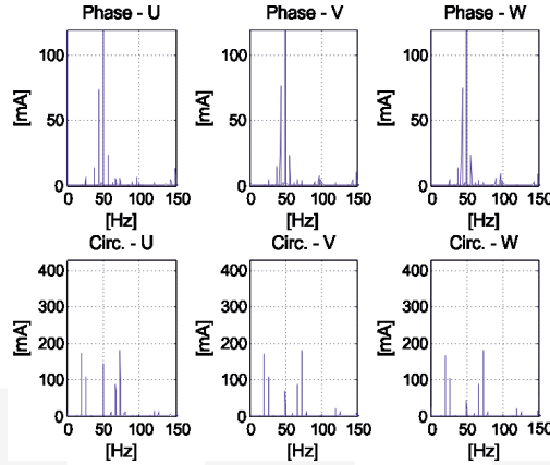
Fig. 6. Harmonics of the phase and circulation currents [mA] – case of air-gap symmetry and 2 broken bars and 30% of shorted turns in the stator phase winding coil
