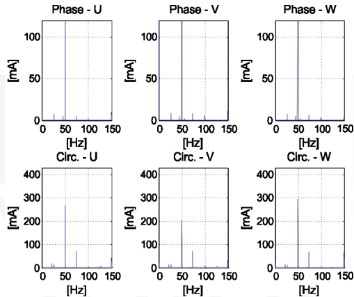
Fig. 7. Harmonics of the phase and circulation currents [mA] – case of 30% static eccentricity and symmetrical stator winding
