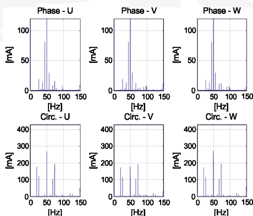
Fig. 9. Harmonics of the phase and circulation currents [mA] – case of 30% static eccentricity and 2 broken bars of the rotor cage and symmetrical stator winding
