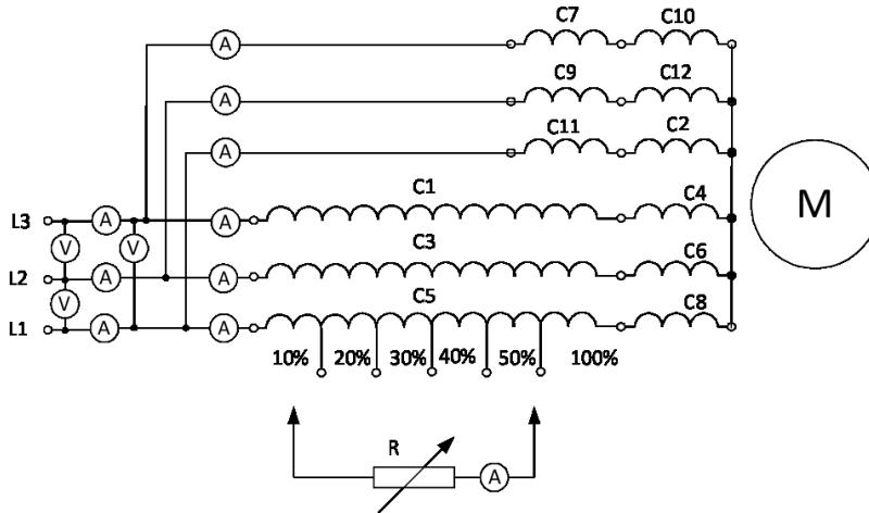
Fig. 2. The wiring diagram of the measuring system
