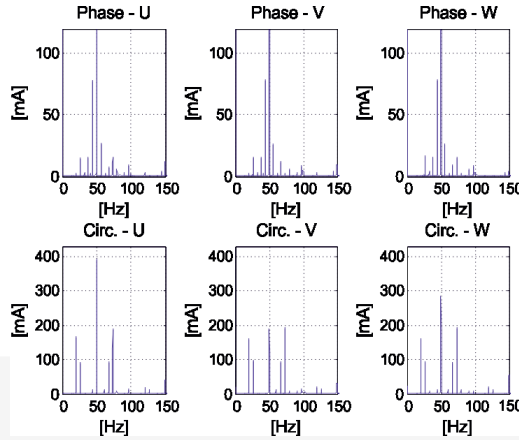
Fig. 10. Harmonics of the phase and circulation currents [mA] – case of 30% static eccentricity and 2 broken bars of the rotor cage and 30% of shorted turns in the coil of the stator phase winding
