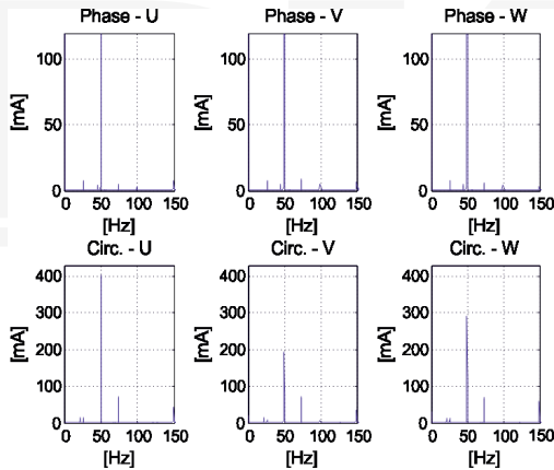
Fig. 8. Harmonics of the phase and circulation currents [mA] – case of 30% static eccentricity and 30% of shorted turns in the stator phase winding coil
