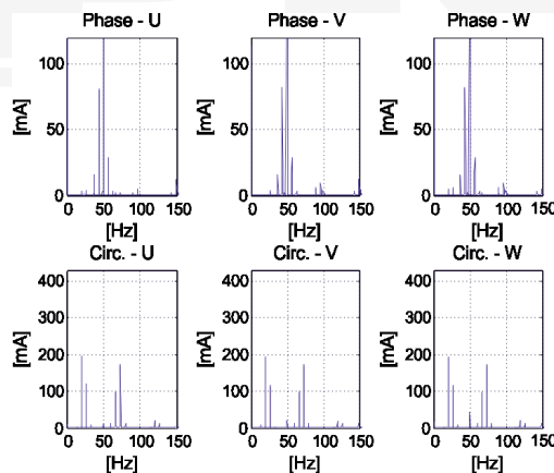
Fig. 5. Harmonics of the phase and circulation currents [mA] – case of air-gap symmetry and 2 broken bars and symmetrical stator winding
