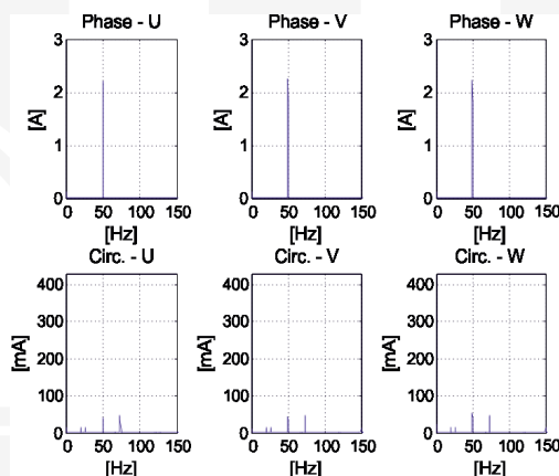
Fig. 3. Harmonics of phase currents [A] (row above) and circulating currents [mA] (row below) – symmetrical machine
