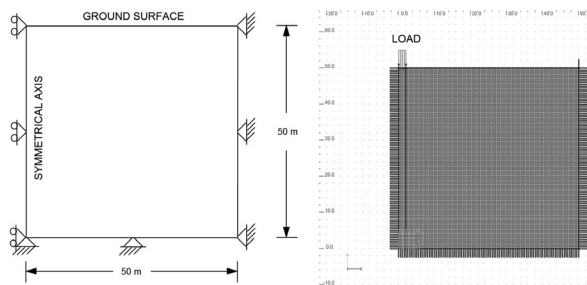
Fig. 2. Boundary conditions for modeling [8] (left), as used in Z_SOIL software suite (right)
