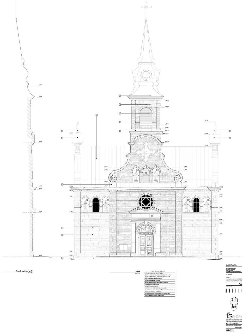
Fig. 6. Parish church in Mystków – main entrance façade and partial section – survey drawings, by Filip Suchoń
