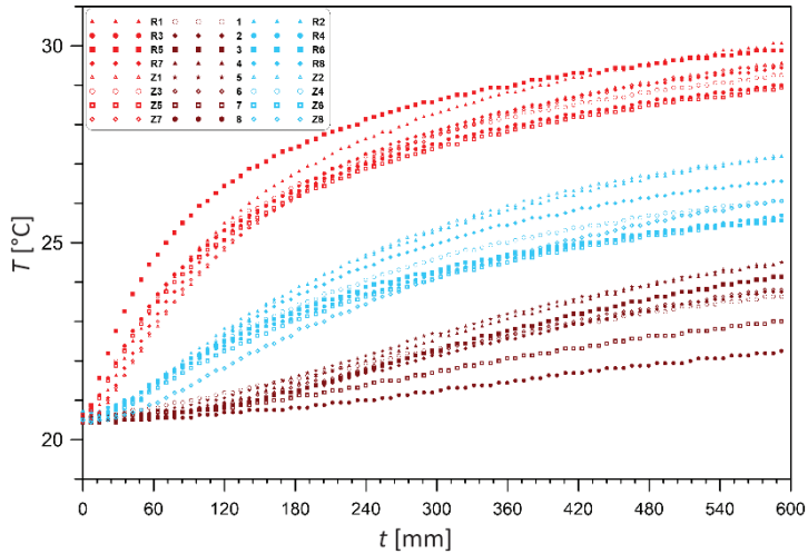
Fig. 5. Measured temporal courses of temperature of granular bed
