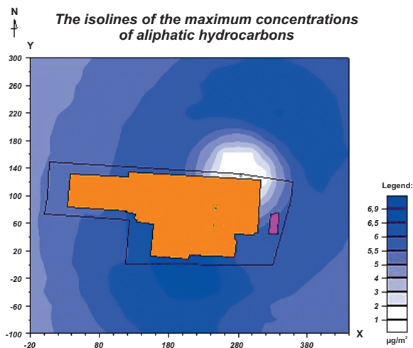
Fig. 2. The drawings present the isolines of the maximum concentrations of selected pollutants
