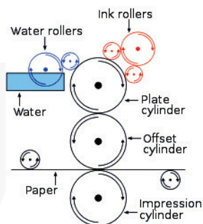
Fig. 1. The principle of offset printing [2]
