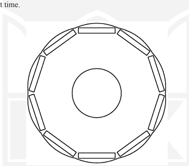
Fig. 2. Investigated 10 poles rotor geometry
