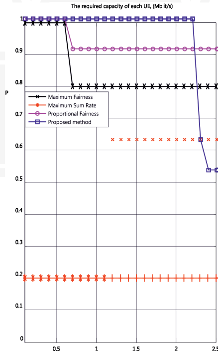
Fig. 3. Dependence of the probability of the required bandwidth capacity allocation to the UE for different methods of frequency-time resource allocation
