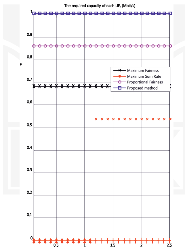
Fig. 2. Dependence of downlink channel bandwidth capacity balancing due to sub-channel allocation method used from the required bandwidth capacity
