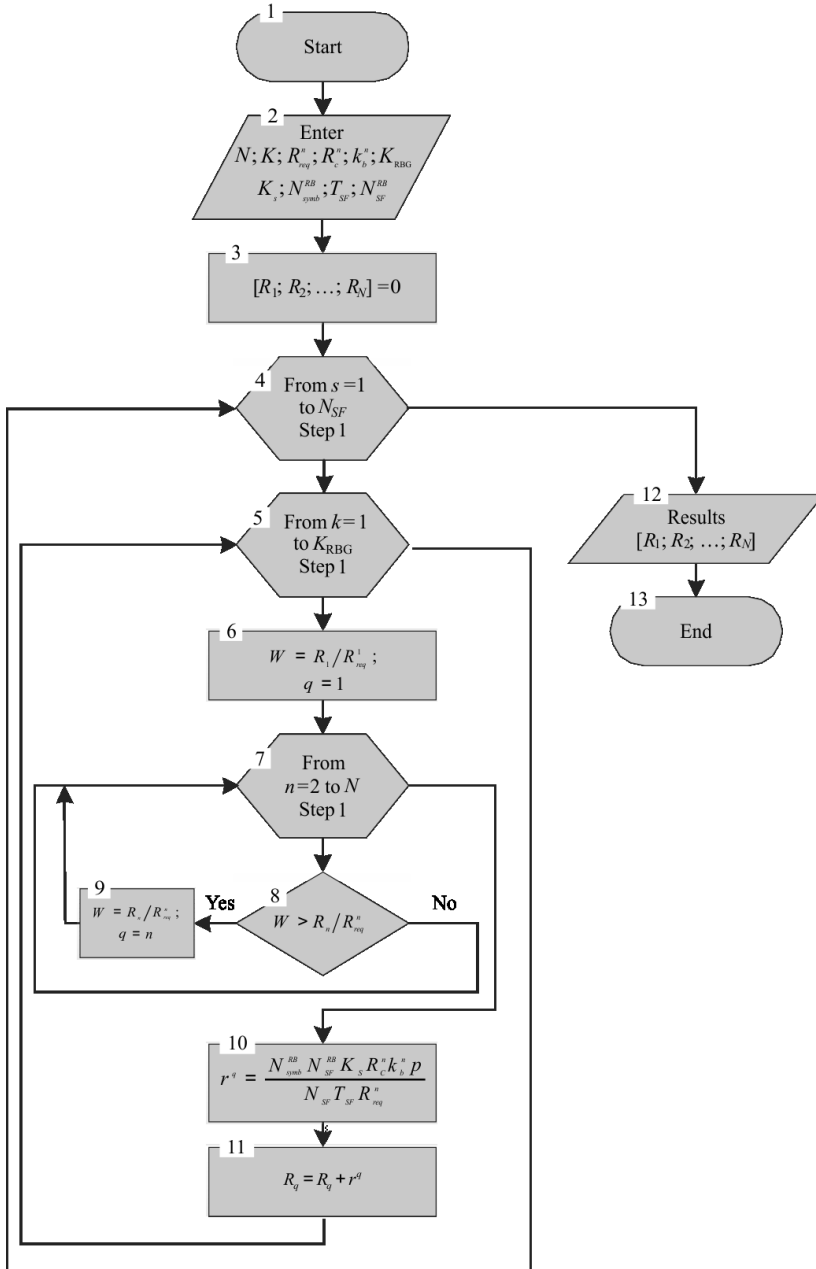
Fig. 1. Flowchart of the algorithm for the proposed method
