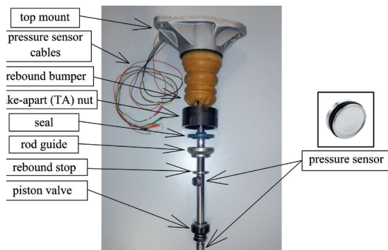
Fig. 3. Instrumented piston rod and top mount unit incl. 4 LC type pressure sensors [11]
