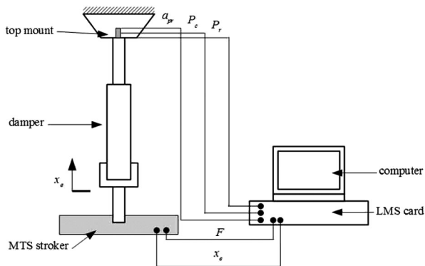
Fig. 2. Measurement system layout. Measured signals: excitation displacement – x_e , piston rod acceleration – a_{pr} , pressure in compression chamber – P_c , pressure in rebound chamber – P_r and damping force – F
