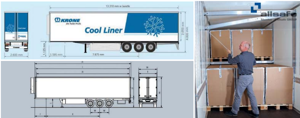
Fig. 3. Dimensions of Krone Cool Liner cooling semi-trailer with ATD II system
