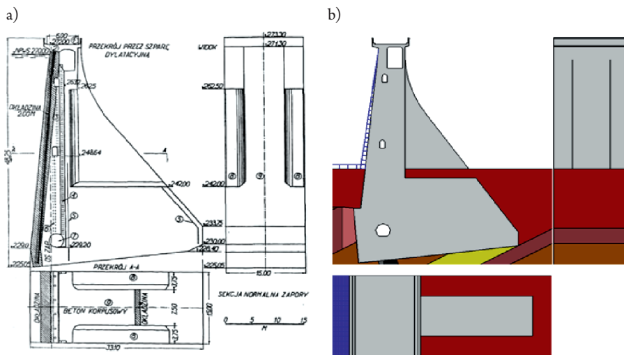
Fig. 2. The geometry of the buttress section: a) sketch [4], b) model generated by Z-Soil software [5]
