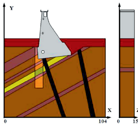
Fig. 3. The geometry and dimensions of the gravity section [5]
