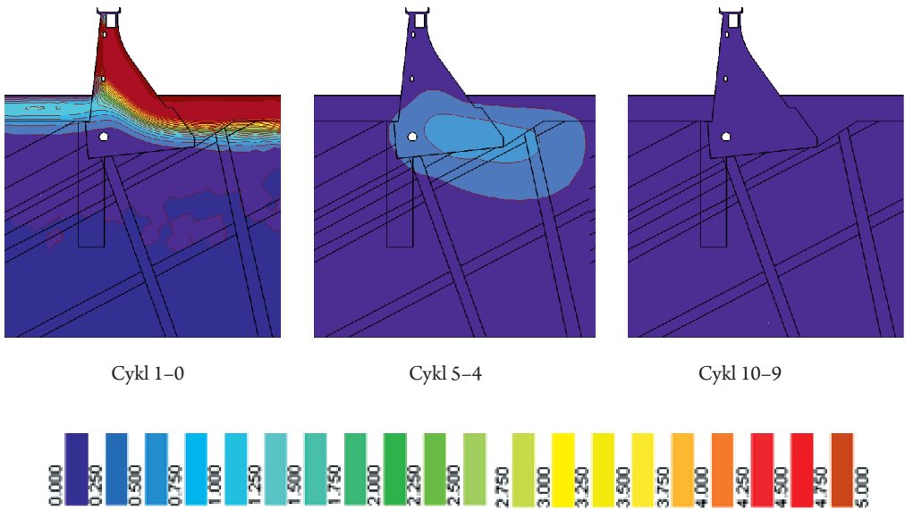
Fig. 7. Changes of temperature in consecutive calculating cycles
