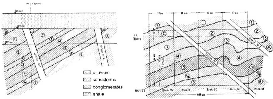
Fig. 1. The system of the geological layers near the 18 th section of the Dam [3]
