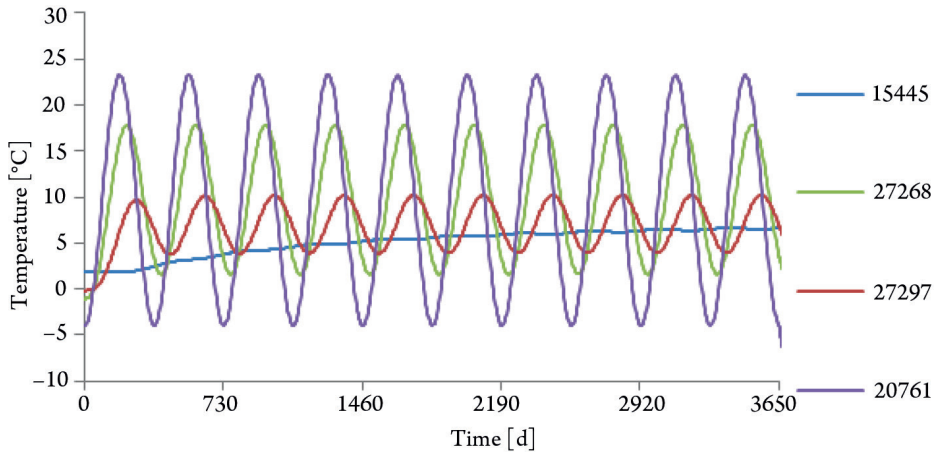
Fig. 10. Temperature changes in time at selected points of the gravity section
