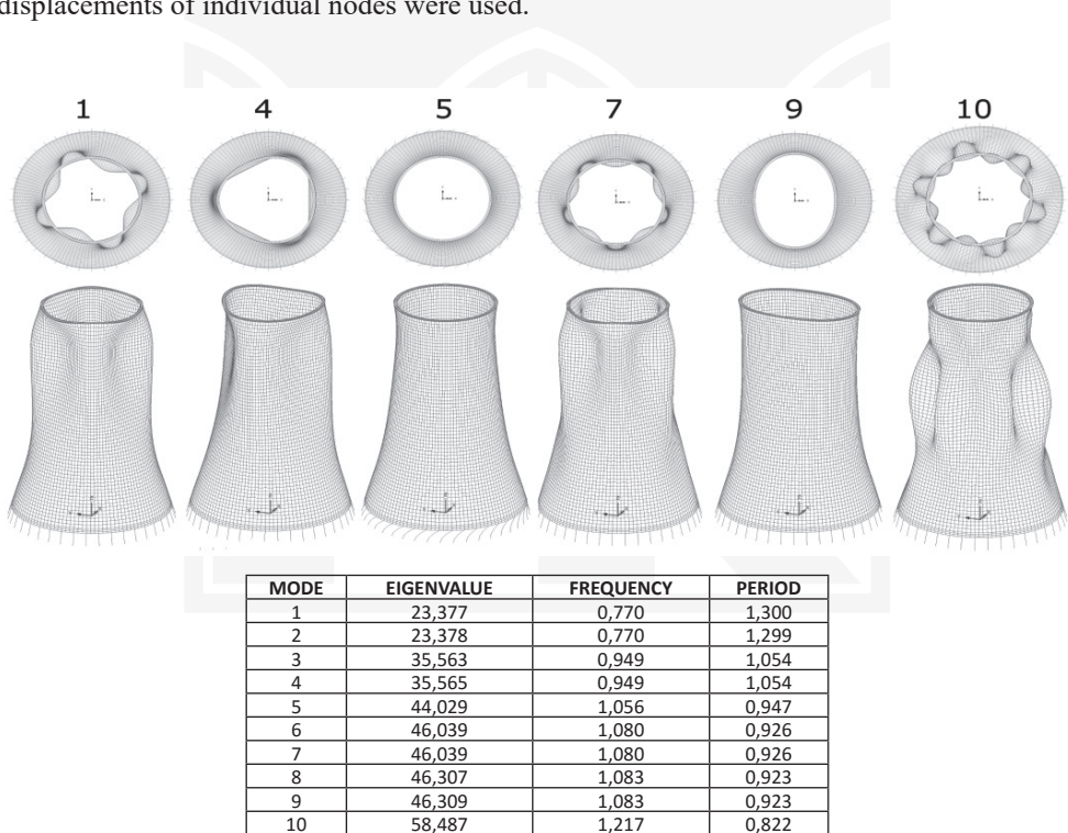
Fig. 5. Natural modes with corresponding eigenvalues and frequency, Lusas [1]
