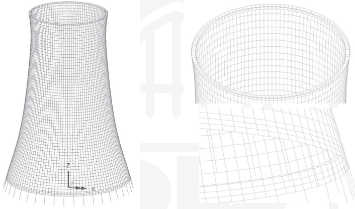
Fig. 1. FEM model and mesh [1]
