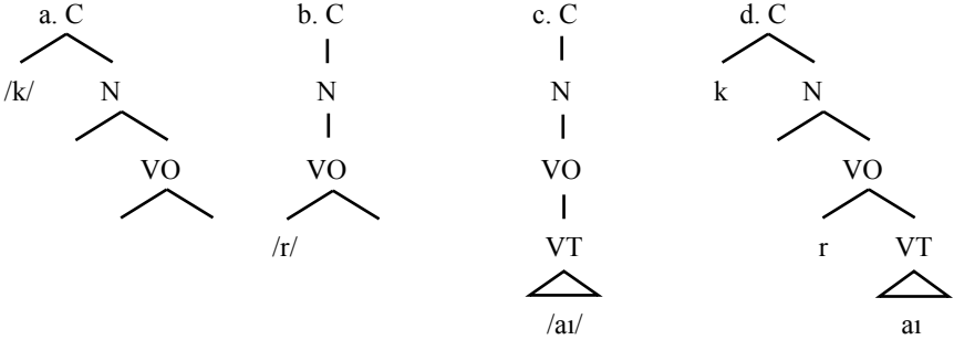
Figure 9. Absorption in English cry
