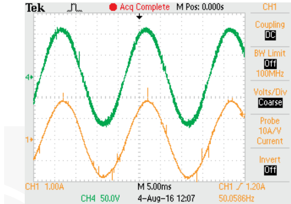
Fig. 10. Phase-to-phase voltage (CH4) and phase current (CH1) waveform after sinusoidal filter from motor side
