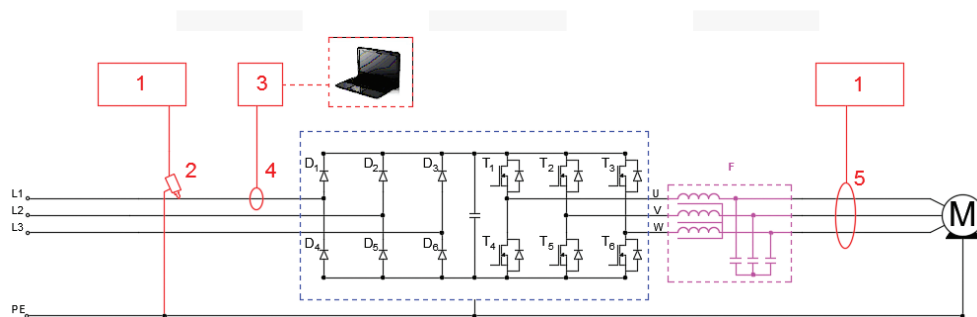
Fig. 1. A simplified measurement setup of converter drive, 1 – spectrum analyzer, 2 – voltage probe, 3 – A/C transducer, 4 – current probe HZ56, 5 – current probe CSP9160A, F – sinusoidal filter
