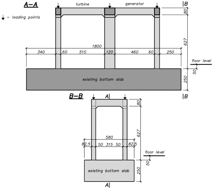
Fig. 2. Longitudinal view and cross-section (dimensions in cm)
