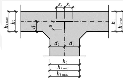
Fig. 4. The node of the structure with rigid sections
