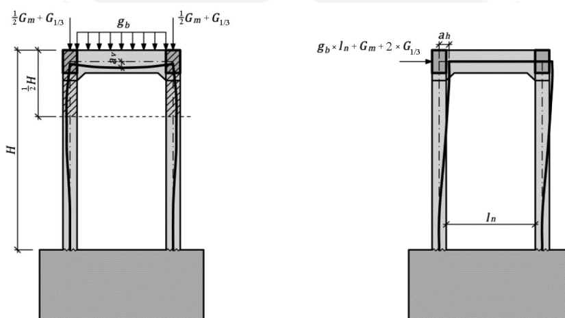
Fig. 3. Diagram for simplified calculations: a) for vertical vibrations, b) for horizontal vibrations
