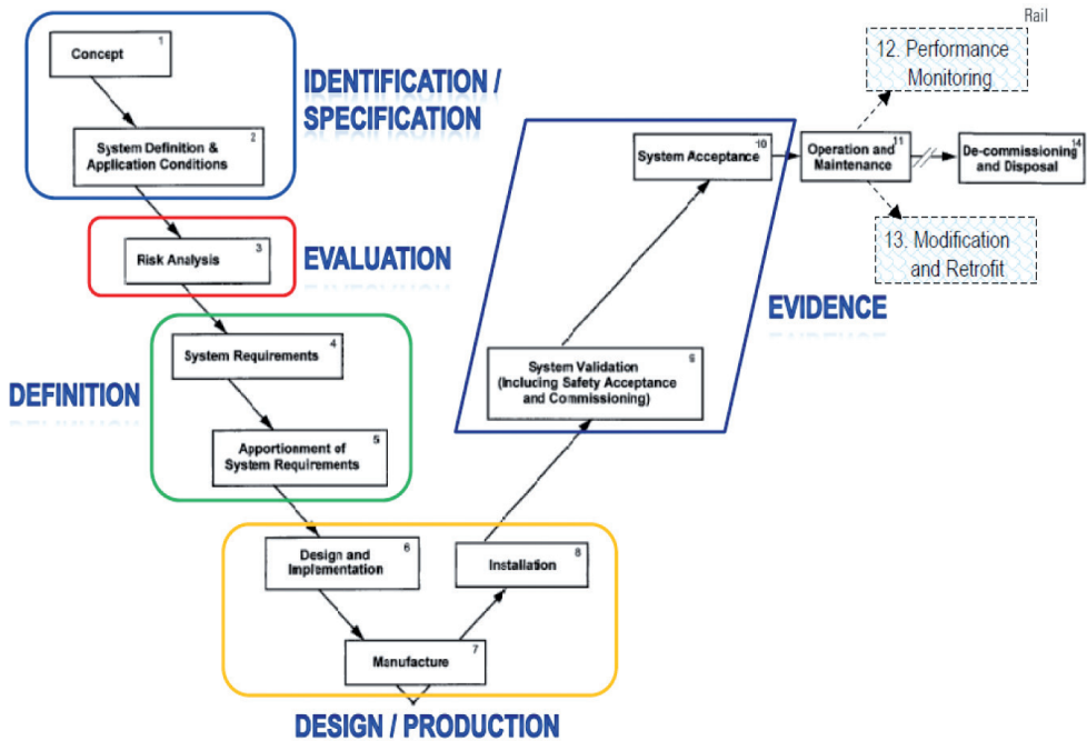
Fig. 5. The V model of project management proposed in the EN50126 standards
