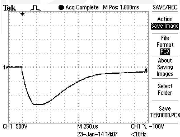
Fig. 9. The voltage waveform U(t) on the terminals of phase B after switching off the current I = 50 mA
