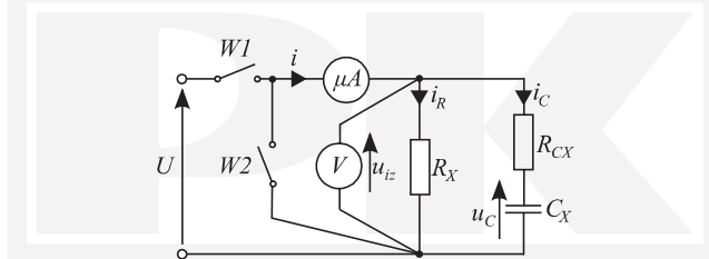
Fig. 5. Interpretation of the charging and discharging of the insulation
