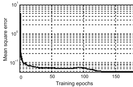
Fig. 3. Graph of the mean square error during the training process
