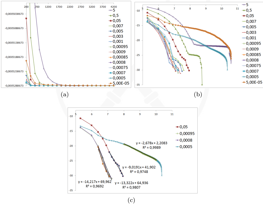
Fig. 7. The convergence history for various u_k values for the mesh 40 \times 4 . The graph (a) shows the iteration number (x axis) vs the objective value (y axis). The same graph with the logarithmic scale for both axes is depicted in the graph (b). Selected plots with fitted lines on the logarithmic scale are depicted in the graph (c)
